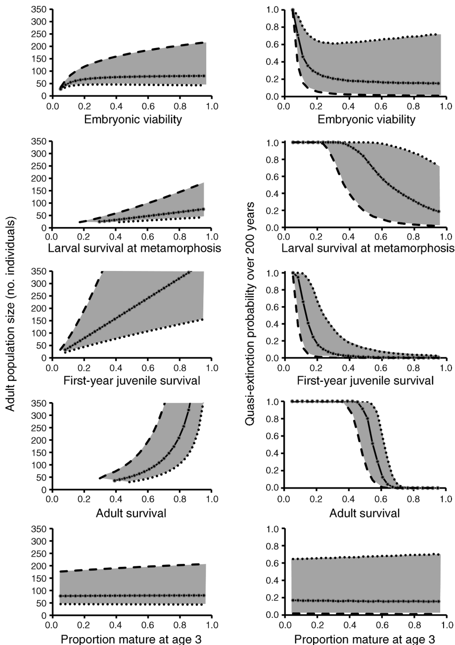
FIG. 1. Sensitivity of Bufo americanus population dynamics to shifts in stage-specific vital rates. Solid isoclines represent mean annual adult population size and quasi-extinction probability as vital rates were varied from 0 to 1 at the mean strength of density dependence ( \gamma = 1 ; Vonesh and De la Cruz 2002). In each case, sensitivity to larval density dependence is indicated by the shaded region, bounded by the confidence interval for \gamma ( \gamma = 1.26 [dotted isoclines], \gamma = 0.76 [dashed isoclines]; Vonesh and De la Cruz 2002). Larval survival at metamorphosis refers to additional mortality occurring at metamorphic climax (i.e., after density effects) when larval density was high ( L_t > 150/m of shoreline; see methods). More steeply sloped isoclines indicate stronger sensitivity of population dynamics to shifting vital rates, whereas flatter isoclines indicate relatively insensitive relationships.
