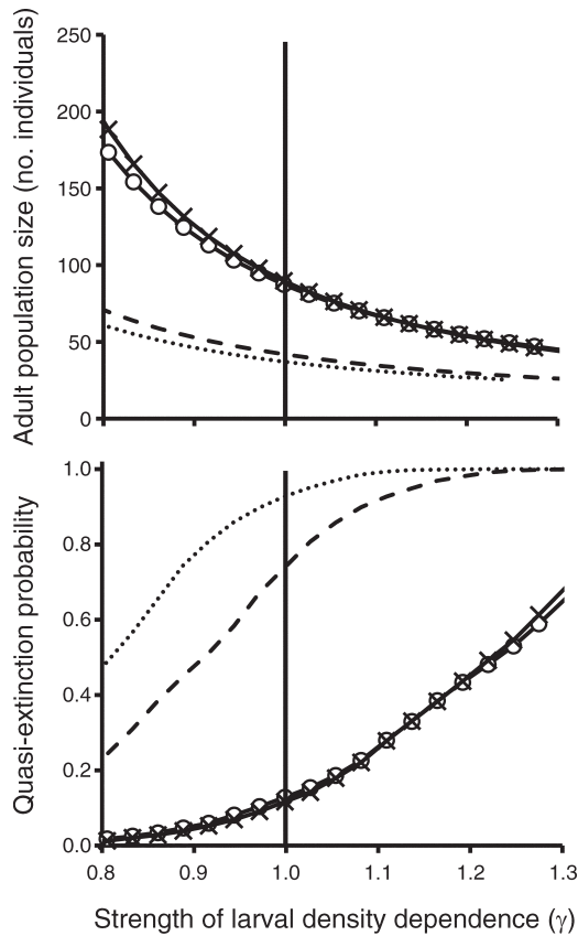
FIG. 2. Case studies evaluating the individual and interactive effects of Hg exposure through maternal transfer and larval diet on Bufo americanus population dynamics. We considered cases of no Hg exposure (solid line), maternal Hg exposure alone (crosses), exposure to Hg through larval diet alone (open circles), and combined maternal and dietary exposure (dashed line), by adjusting model parameters based on all observed Hg effects for each exposure scenario (Table 1). Additionally, we considered a hypothetical case where maternal and dietary Hg exposure resulted in minor additional adult mortality (5% reduction in survival; dotted line). We examined the effects of Hg exposure on quasi-extinction probability and mean annual adult population size for each case across varying strengths of density dependence ( \gamma ; 95% CI for B. americanus = 0.76–1.26; mean = 1 [solid vertical line]; Vonesh and De la Cruz 2002).
